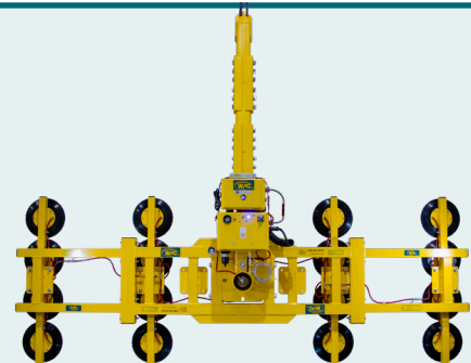
MR1611LDC (refer to Spec Sheet 6-4 for specifications)
