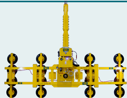
MR1611LDC (refer to Spec Sheet 6-4 for specifications)
