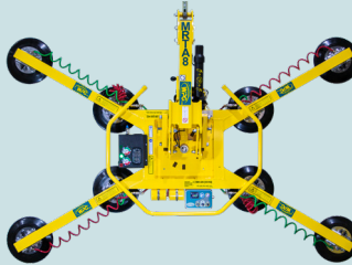
MRTA811LDC3 (refer to Spec Sheet 8-8 for specifications)
